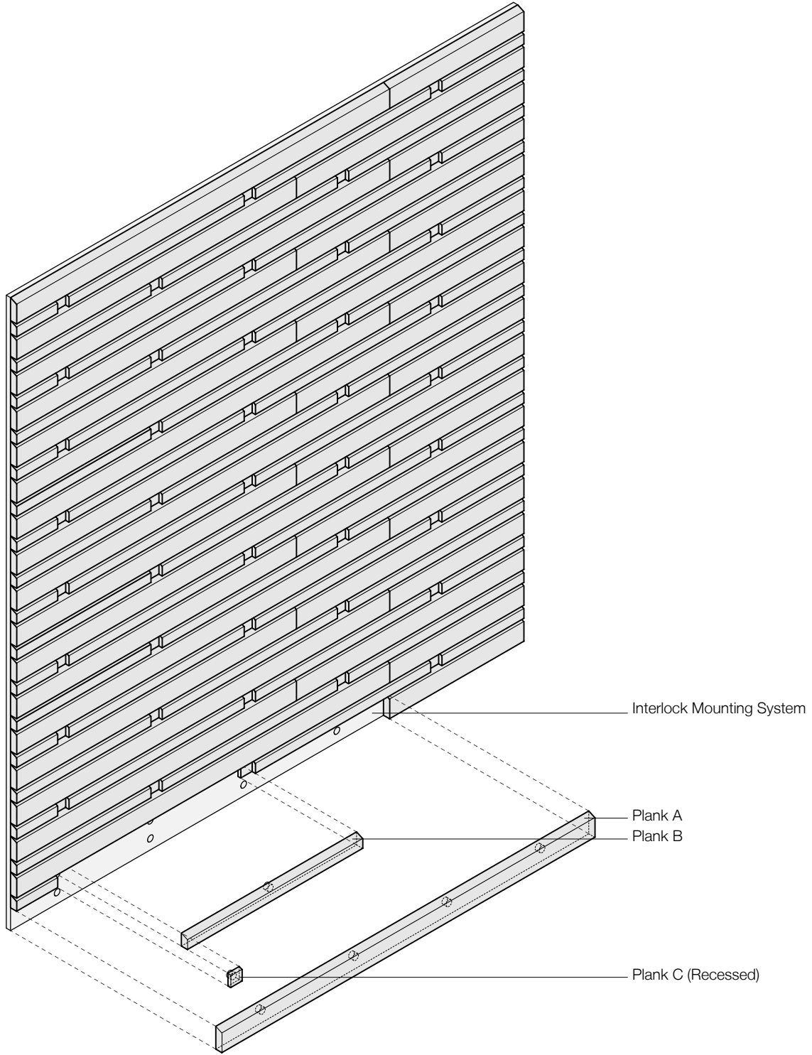
Exploded Axonometric
