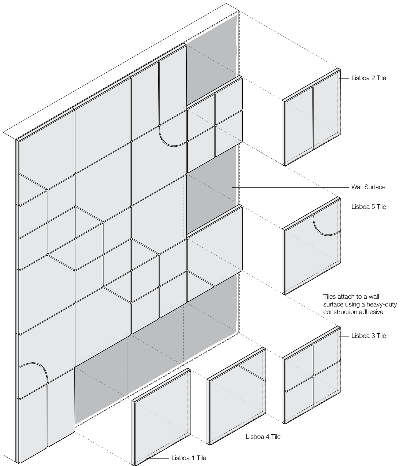
Exploded Axonometric
