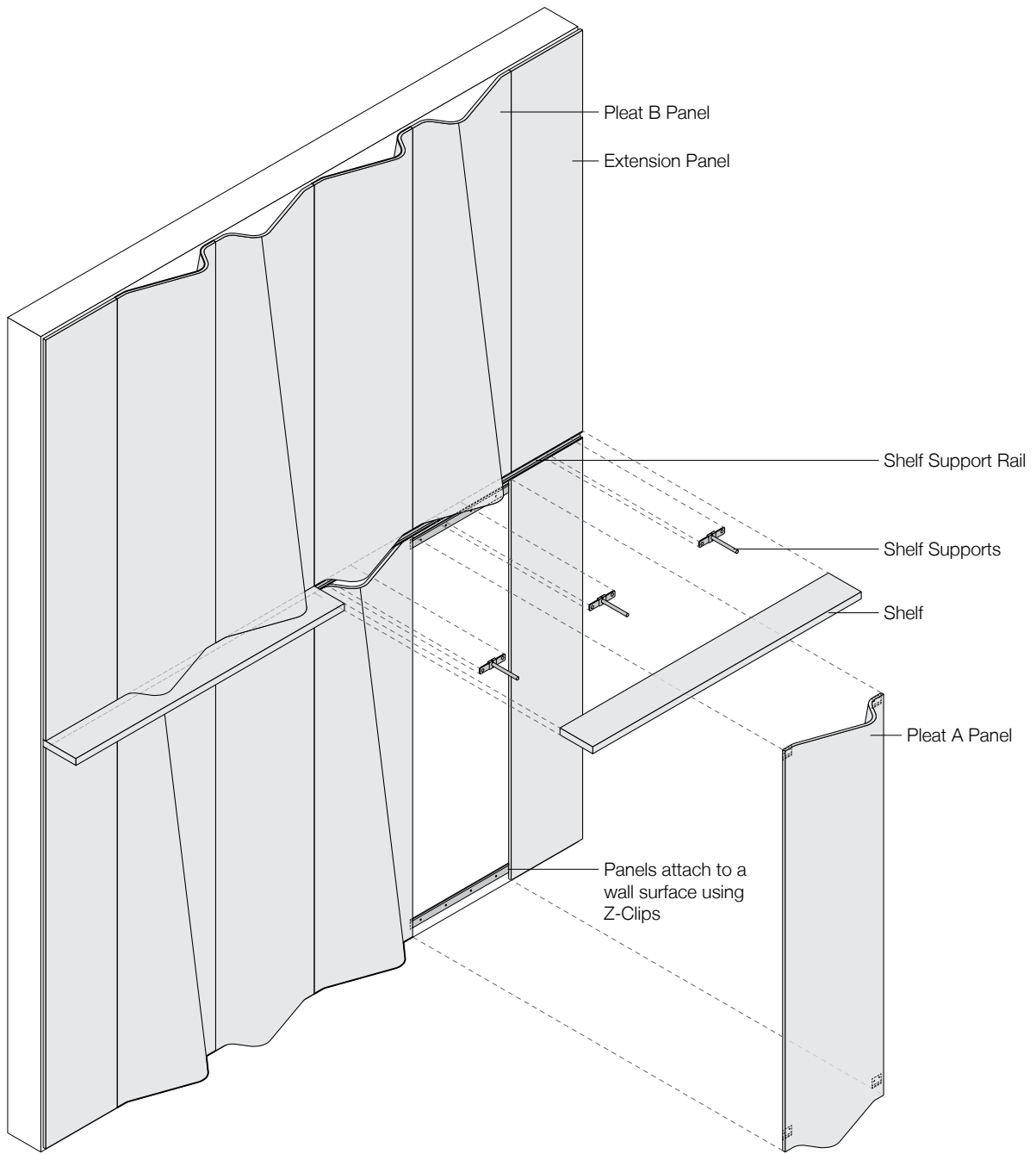
Exploded Axonometric
